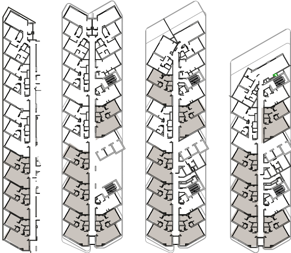
LEVEL 1-9, 12-13
