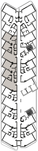
LEVEL 1-9
